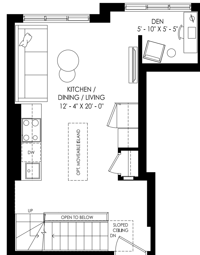
FIFTH FLOOR
