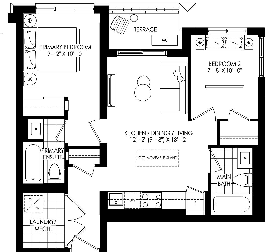
THIRD FLOOR
