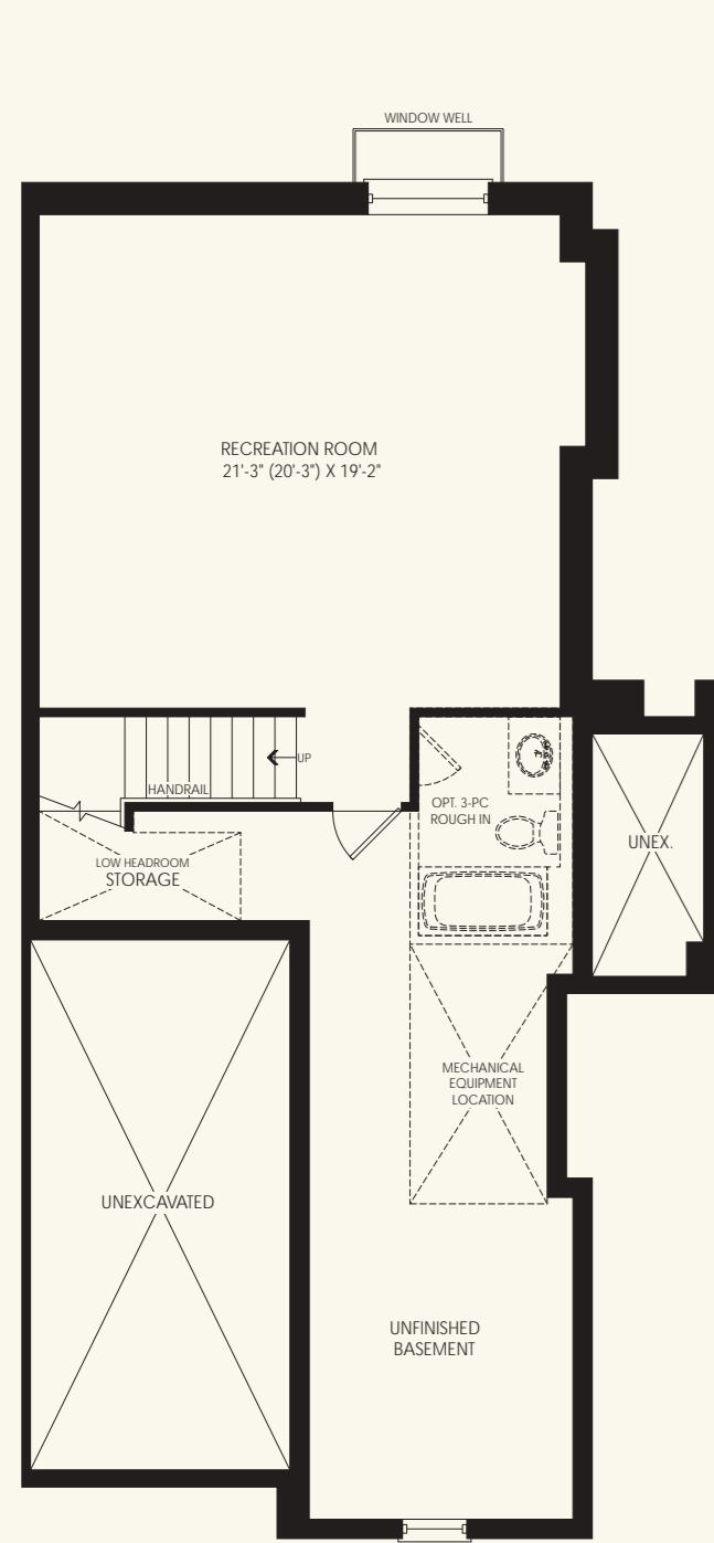
FINISHED BASEMENT PLAN W/ RECREATION ROOM ELEV 'A'
