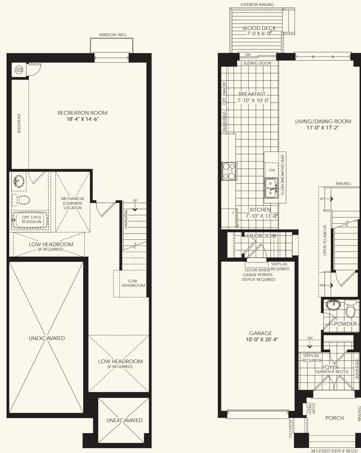
BASEMENT PLAN ELEV 'A'
