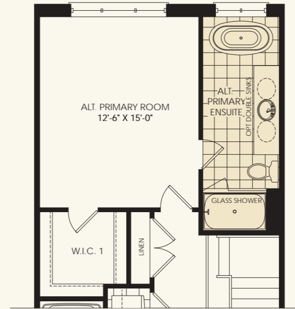
PARTIAL OPT. SECOND FLOOR PLAN W/ ALT. PRIMARY BEDROOM & ALT. PRIMARY ENSUITE ELEV. 'A'
