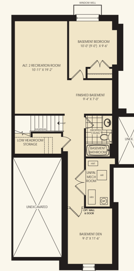
OPTION 2 FINISHED BASEMENT PLAN W/ ALT. RECREATION ROOM, BASEMENT BEDROOM, BASEMENT BATH & DEN ELEV 'A' (IF GRADE PERMITS)
