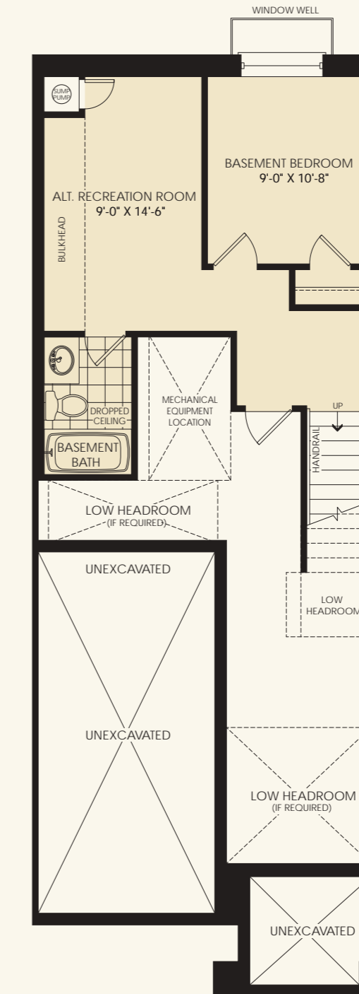
OPT. BASEMENT PLAN W/ ALT. REC ROOM, BASEMENT BEDROOM & BASEMENT BATHROOM ELEV. 'A' IF GRADE PERMITS
