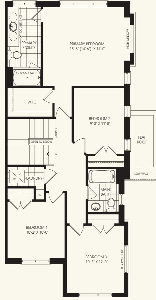
SECOND FLOOR PLAN ELEV 'A'
