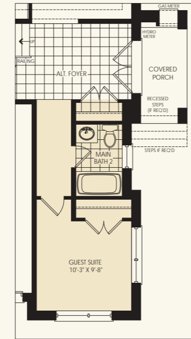
PARTIAL OPT. GROUND FLOOR PLAN W/ GUEST SUITE ELEV 'A'
