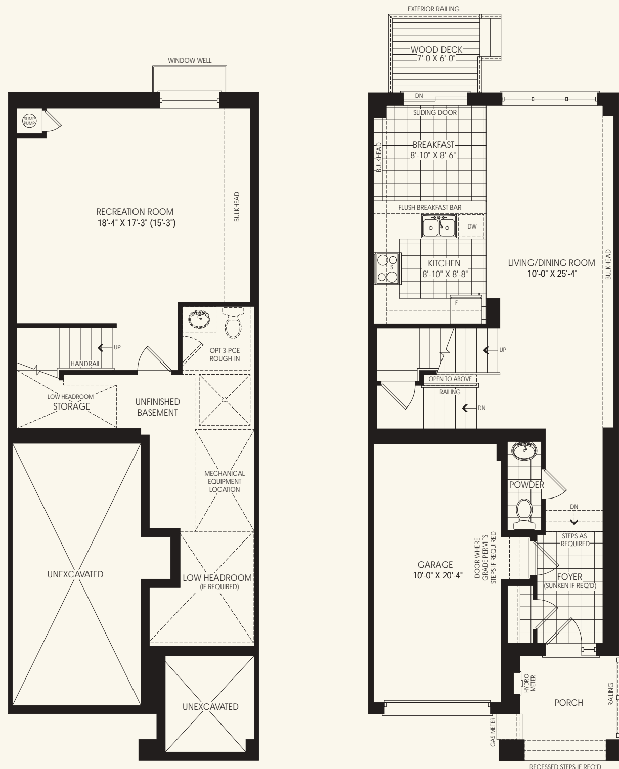
GROUND FLOOR PLAN ELEV 'A'
