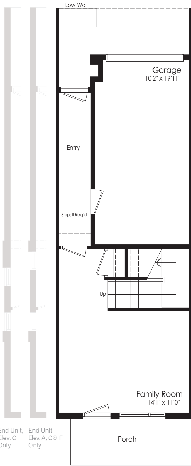
End Unit, Elev. G Only End Unit, Elev. A, C & F Only Main Level
