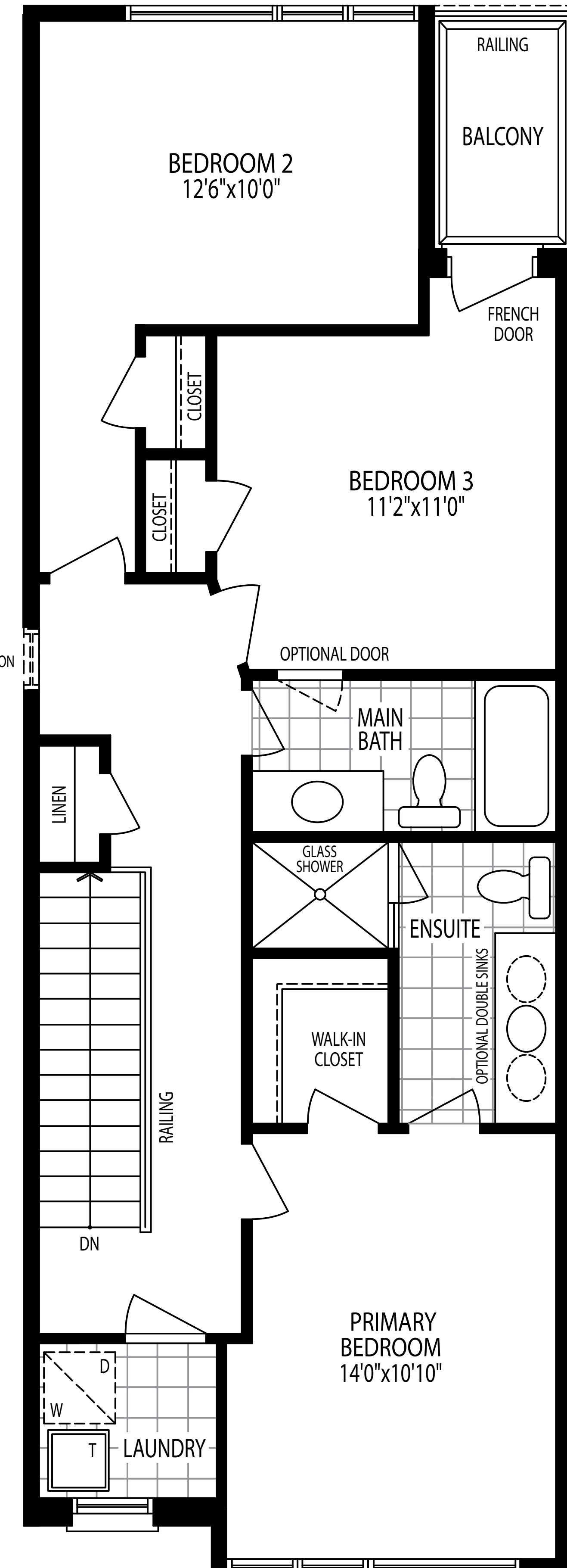
UPPER FLOOR PLAN ELEV. A
