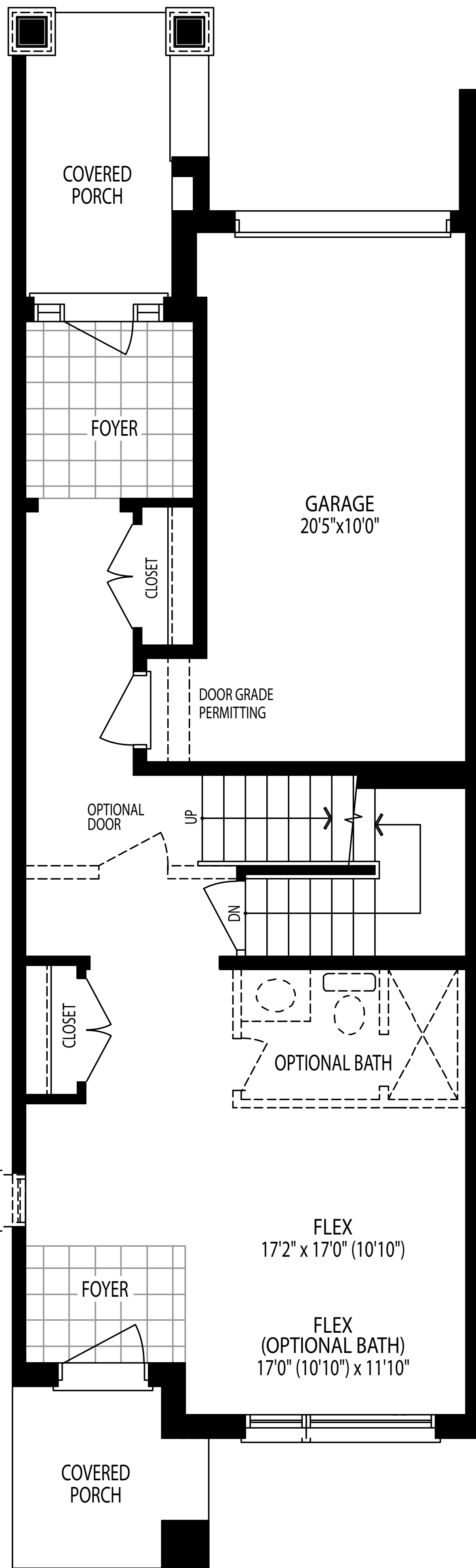
GROUND FLOOR PLAN ELEV. A
