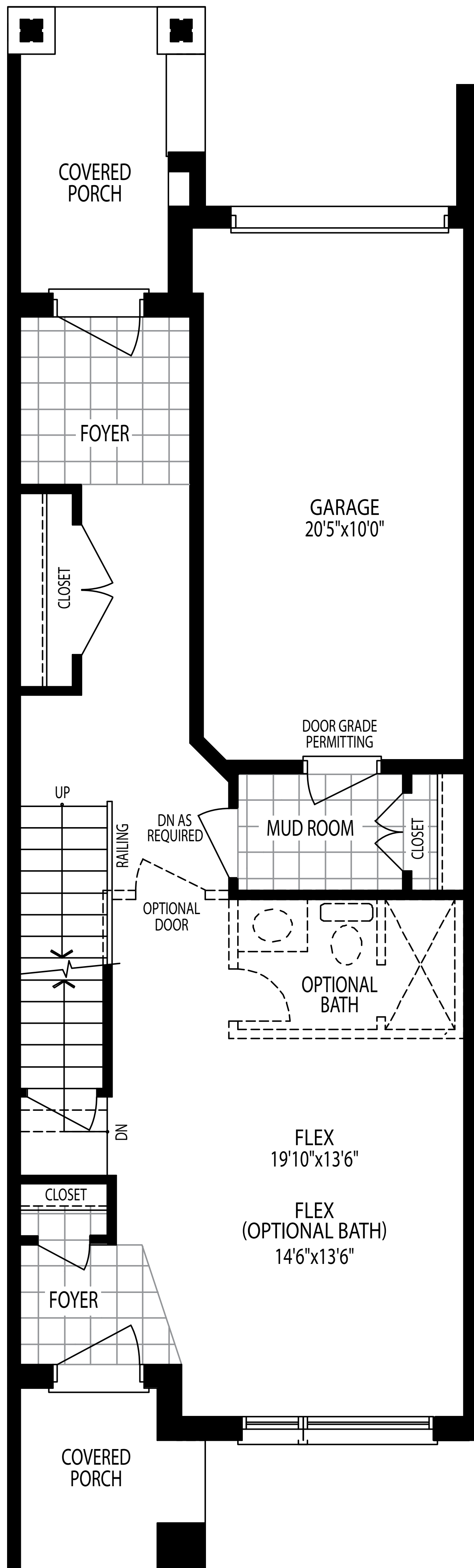
GROUND FLOOR PLAN ELEV. A
