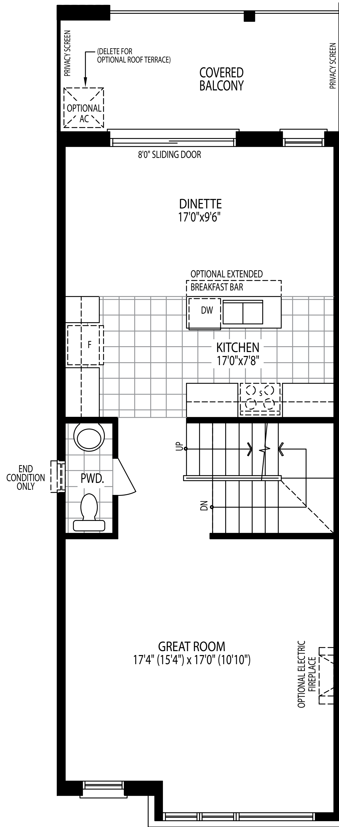
MAIN FLOOR PLAN ELEV. A
