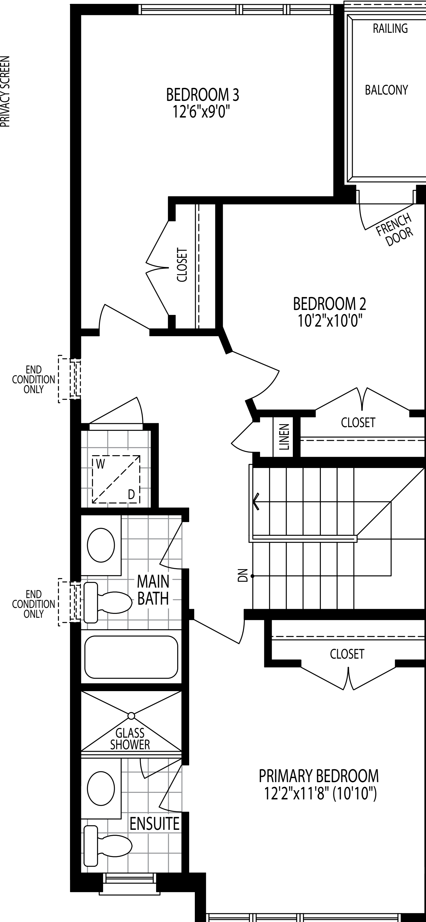
UPPER FLOOR PLAN ELEV. A
