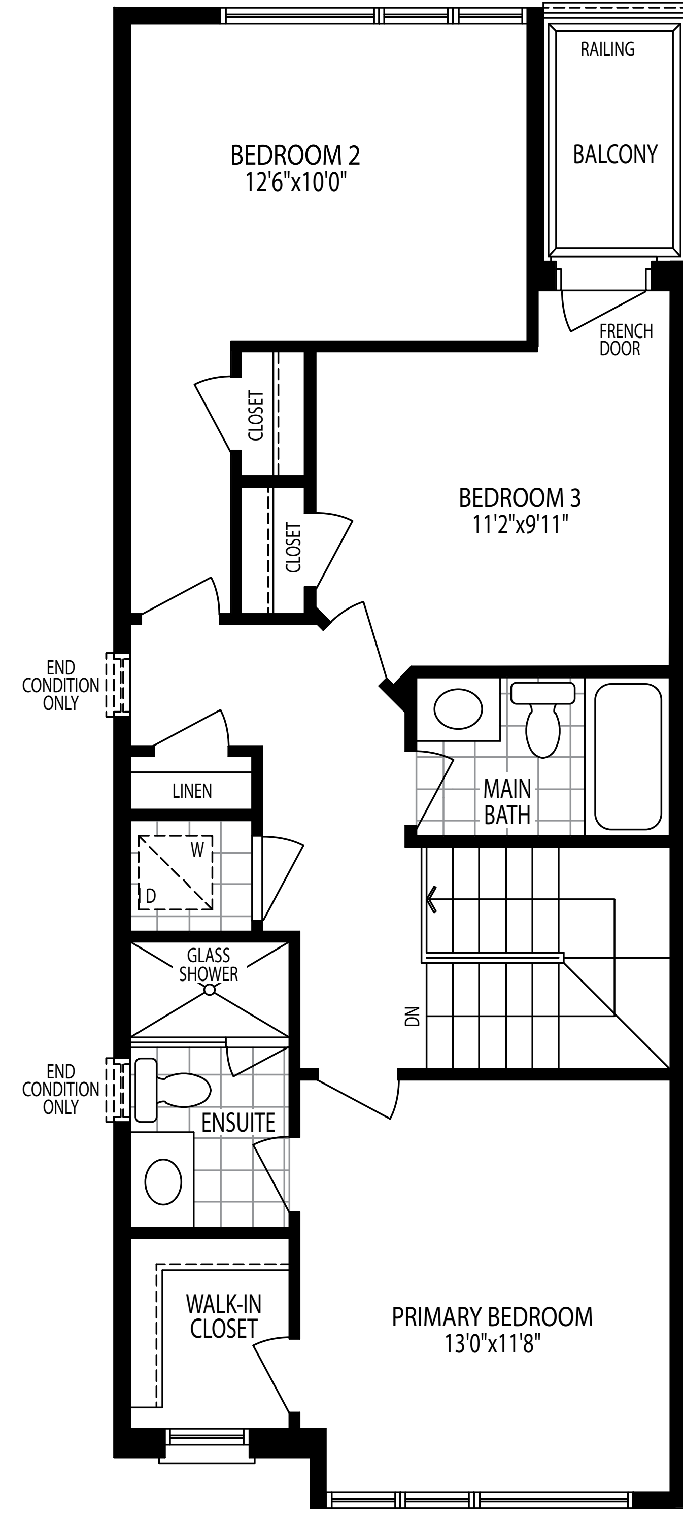
UPPER FLOOR PLAN ELEV. A
