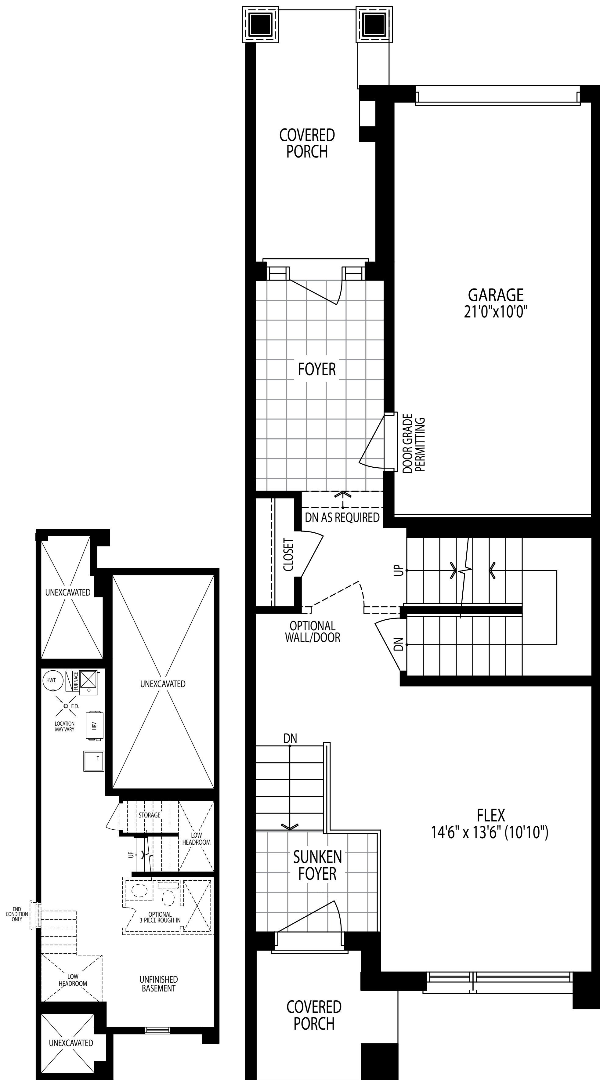
BASEMENT PLAN SUNKEN FRONT FOYER CONDITION ELEV. A
