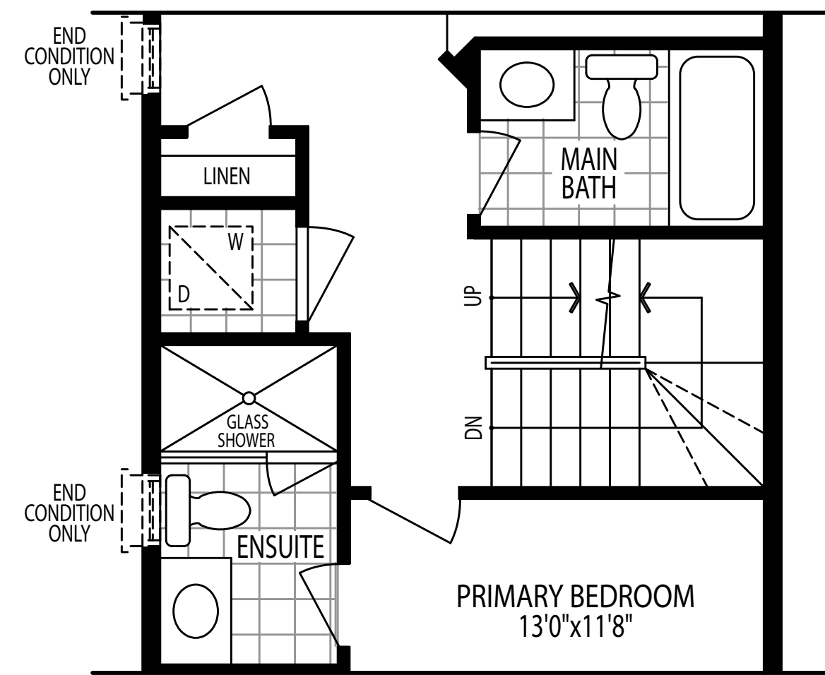
PARTIAL UPPER FLOOR PLAN FOR OPT. ROOF TERRACE ELEV. A
