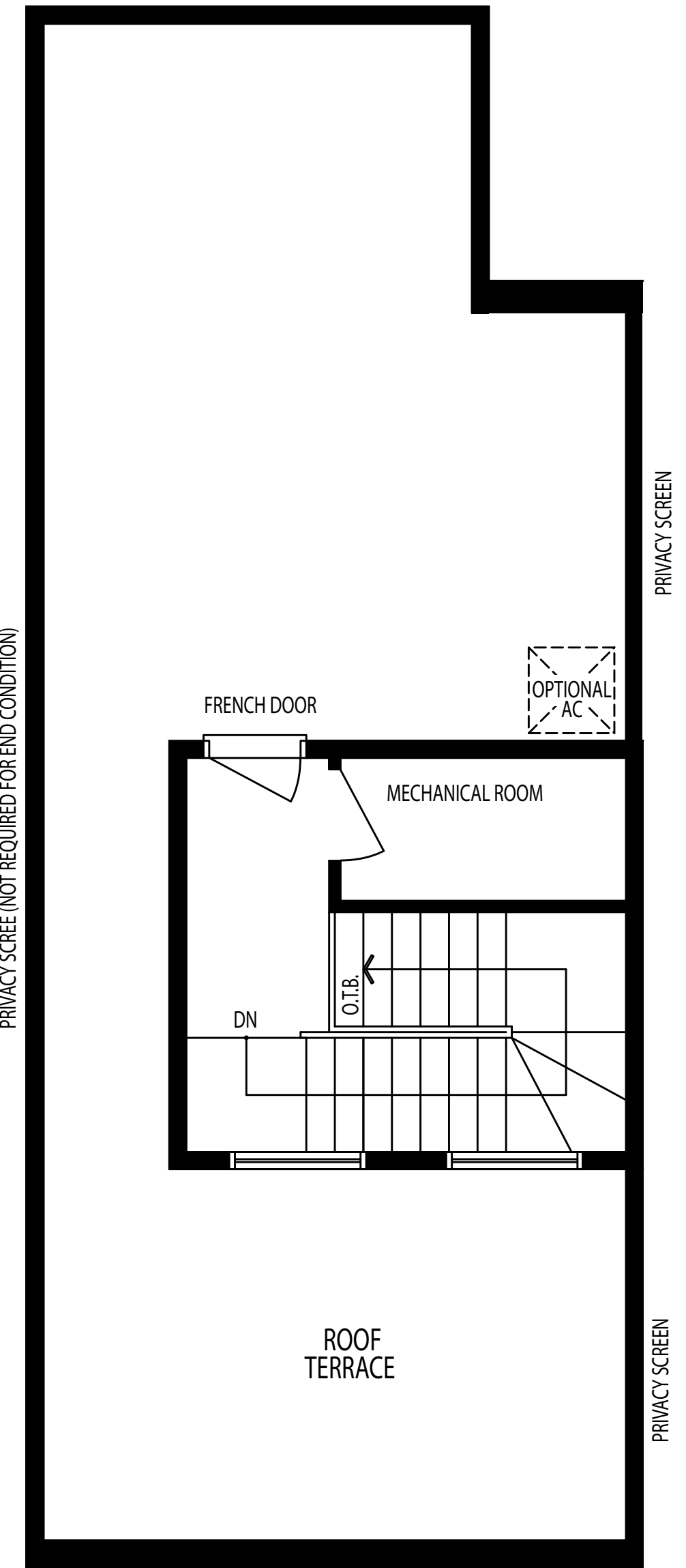
OPT. ROOF TERRACE ELEV. A
