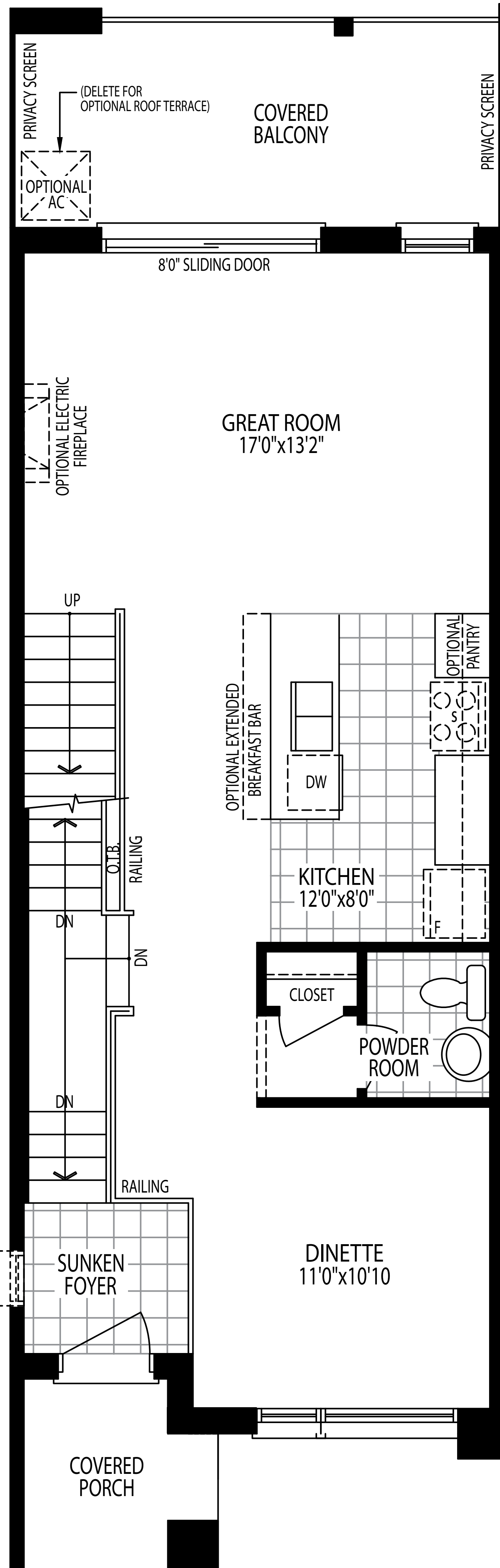
MAIN FLOOR PLAN SUNKEN FRONT FOYER CONDITION ELEV. A
