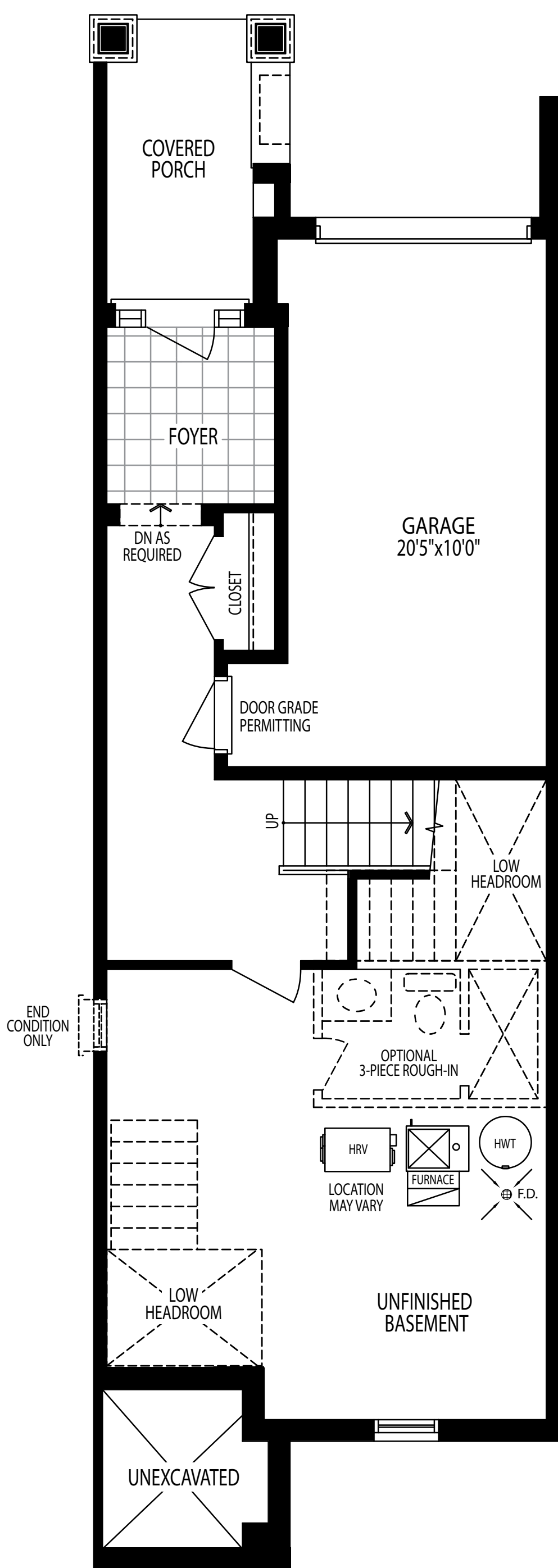
BASEMENT PLAN SUNKEN FRONT FOYER CONDITION ELEV. A
