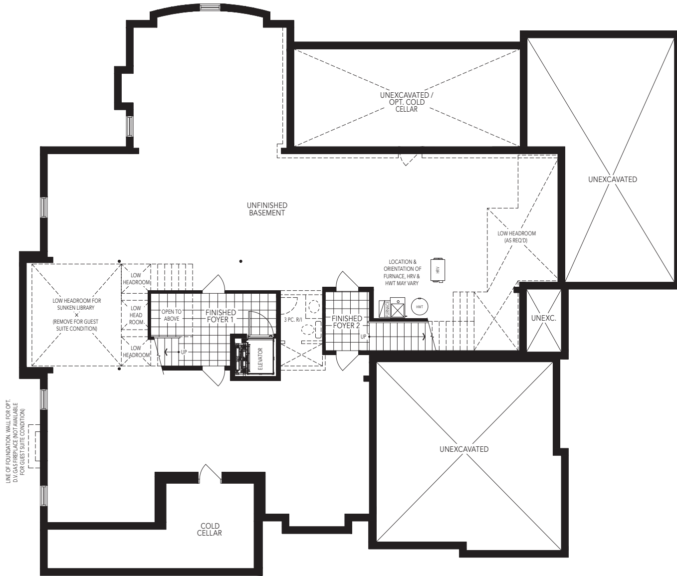
BASEMENT W/OPT. ELEVATOR ELEVATION B
