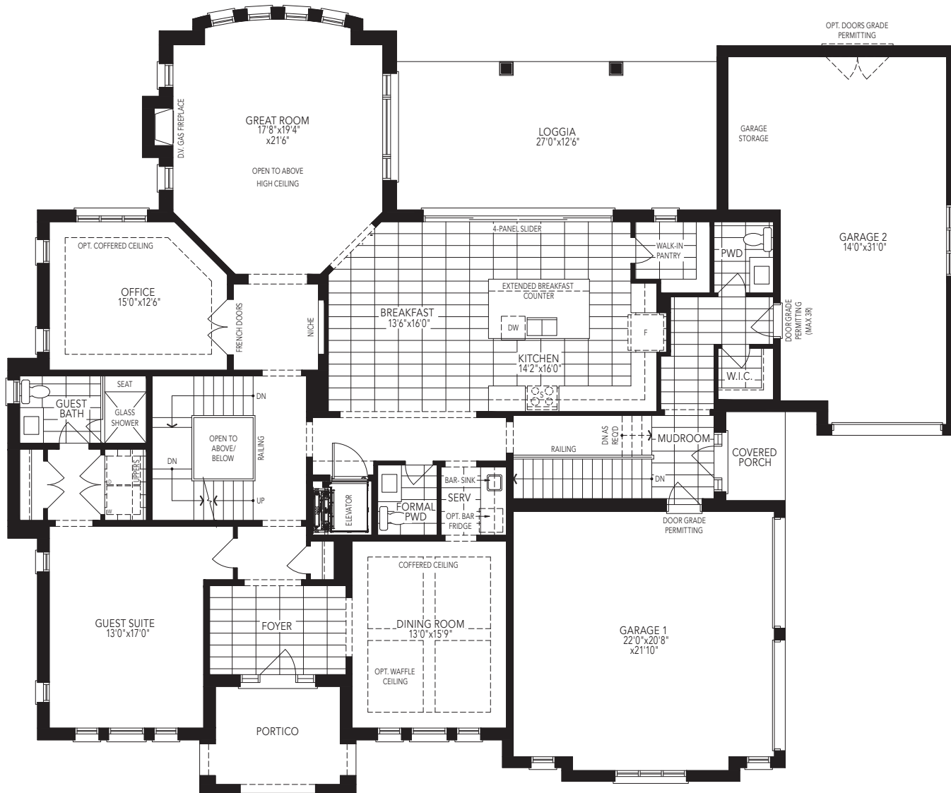
GROUND FLOOR W/OPT. ELEVATOR + GUEST SUITE ELEVATION A
