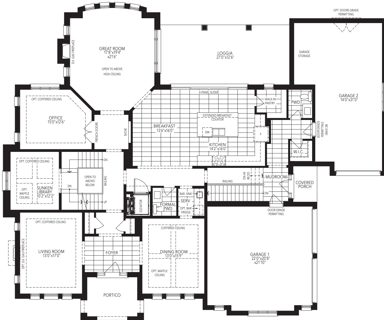
GROUND FLOOR W/OPT. ELEVATOR ELEVATION A
