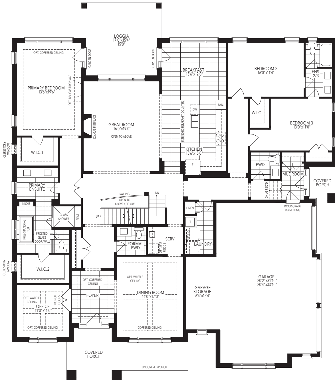
GROUND FLOOR W/OPT. LOFT ELEVATION C
