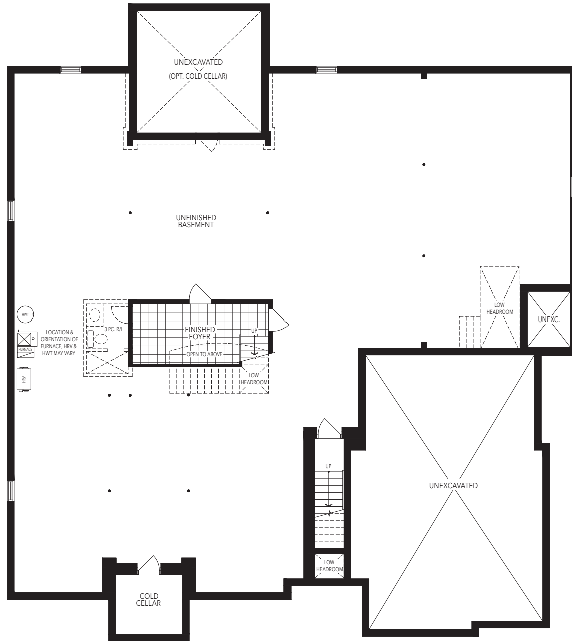
BASEMENT W/ OPT. SERVICE STAIRS ELEVATION B
