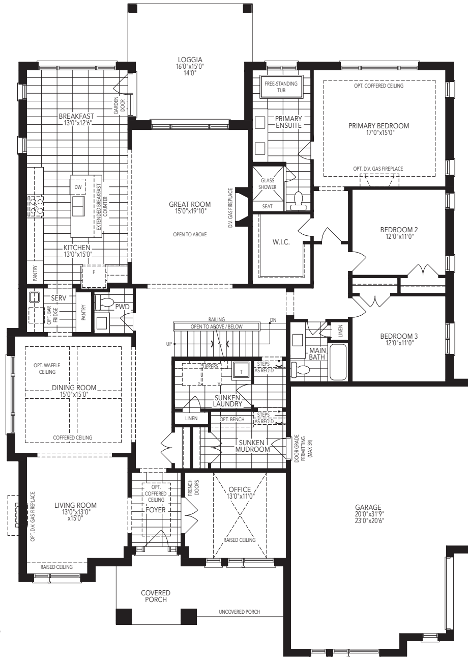
GROUND FLOOR W/OPT. LOFT ELEVATION C
