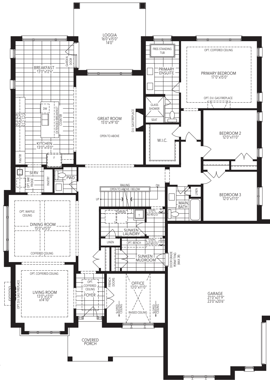
GROUND FLOOR W/OPT. LOFT ELEVATION B
