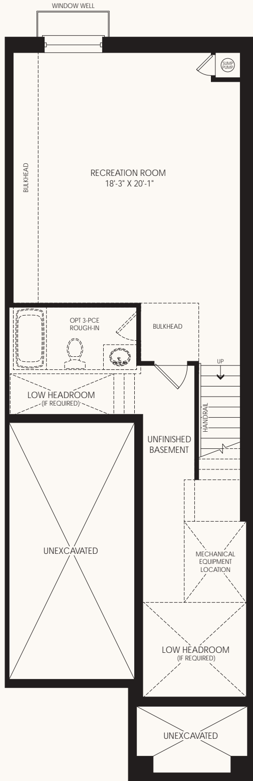
BASEMENT PLAN ELEV. 'A'
