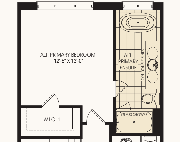
PARTIAL OPT. SECOND FLOOR PLAN W/ ALT. PRIMARY BEDROOM & ALT. PRIMARY ENSUITE ELEV. 'A'
