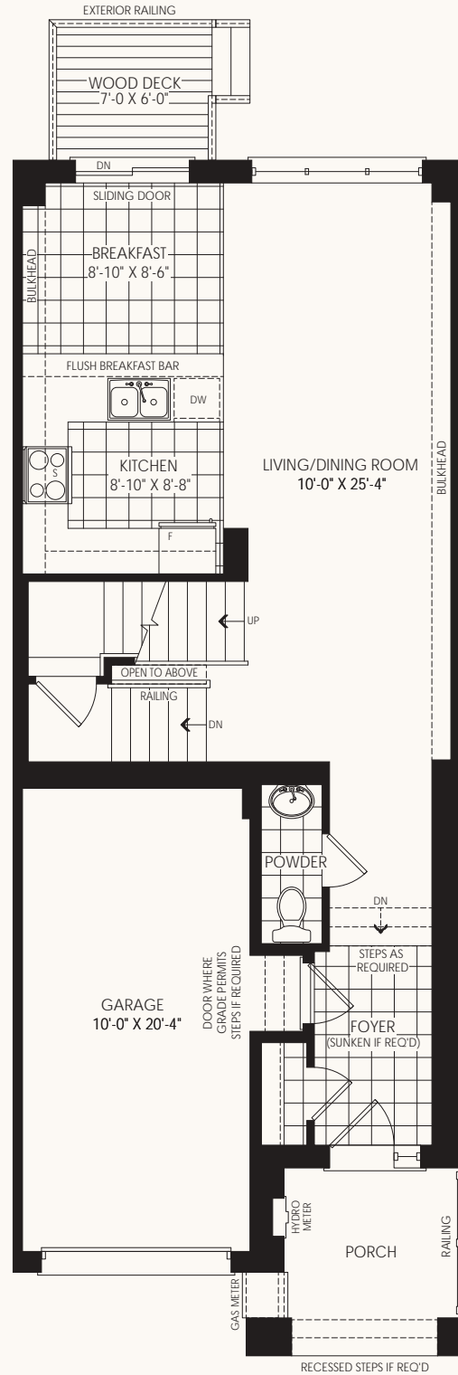
GROUND FLOOR PLAN ELEV 'A'
