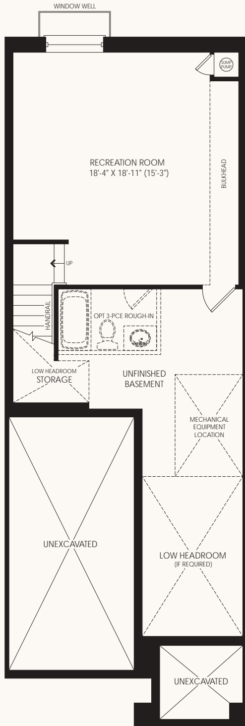
BASEMENT PLAN ELEV 'A'
