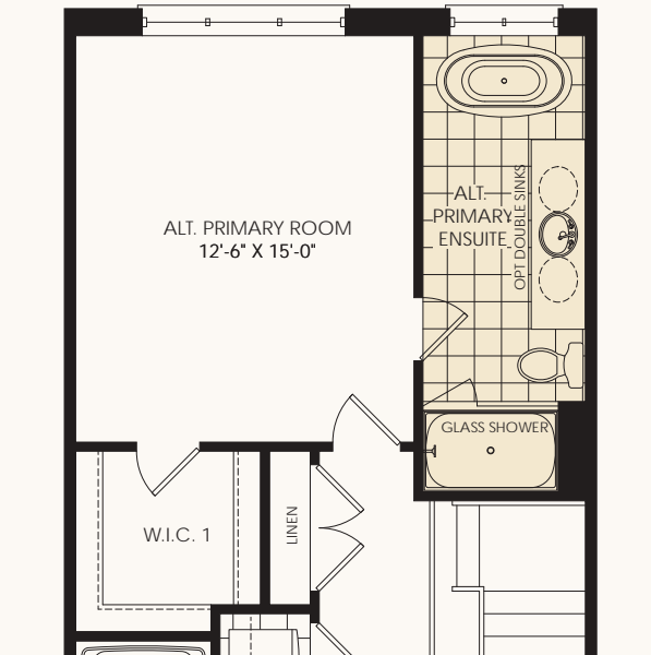
PARTIAL OPT. SECOND FLOOR PLAN W/ ALT. PRIMARY BEDROOM & ALT. PRIMARY ENSUITE ELEV. 'A'
