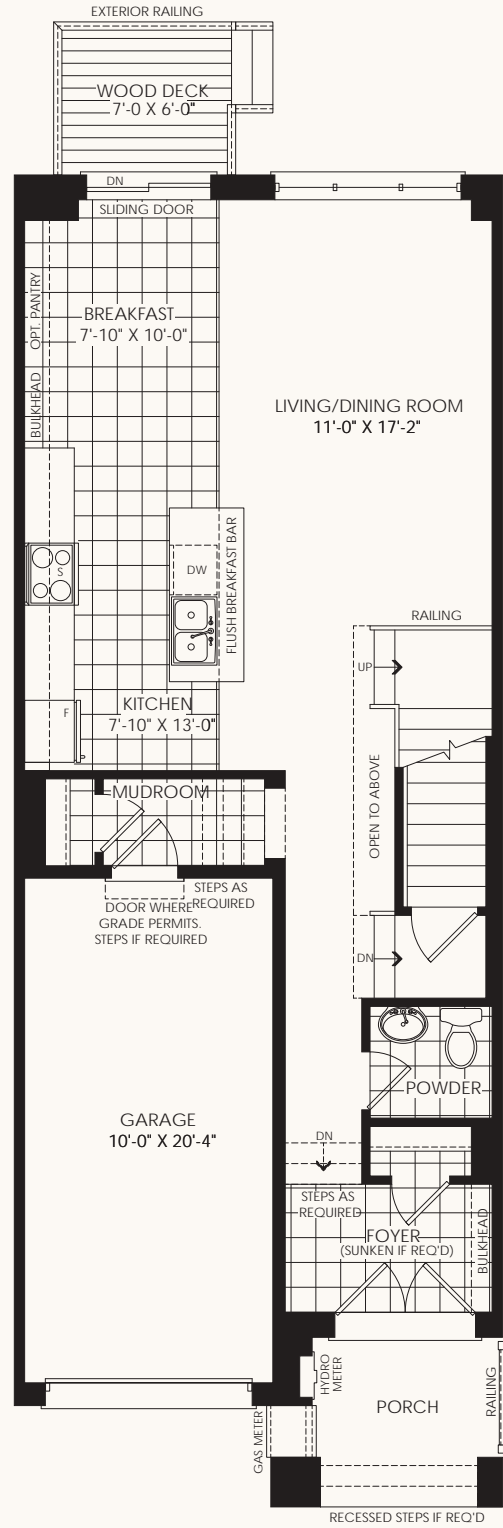
GROUND FLOOR PLAN ELEV 'A'
