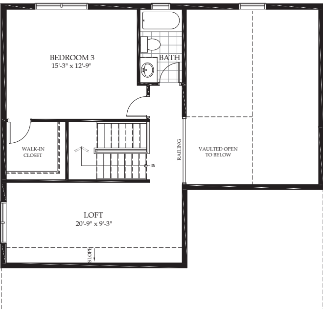
+1 BEDROOM LOFT OPT. B 677 SQ.FT.
