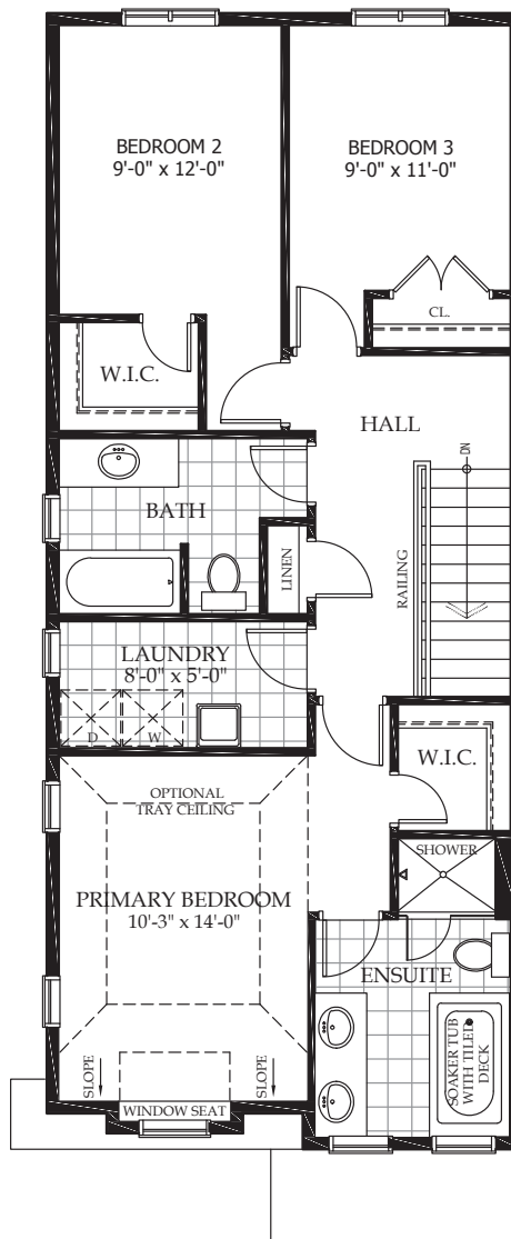
3 BEDROOM - OPT. B UPPER LEVEL 915 SQ.FT.
