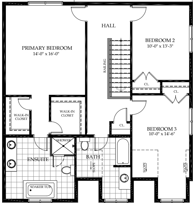
3 BEDROOM UPPER LEVEL 1,175 SQ.FT.
