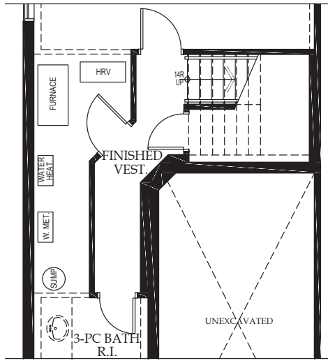
LOWER LEVEL OPTIONAL FINISHED VESTIBULE AREA OF 54 SQ.FT.
