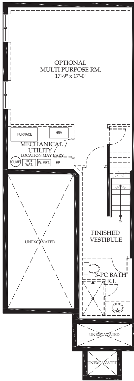
LOWER LEVEL OPTIONAL FINISHED AREA OF 458 SQ.FT. OPTIONAL FINISHED VESTIBULE AREA OF 62 SQ.FT.
