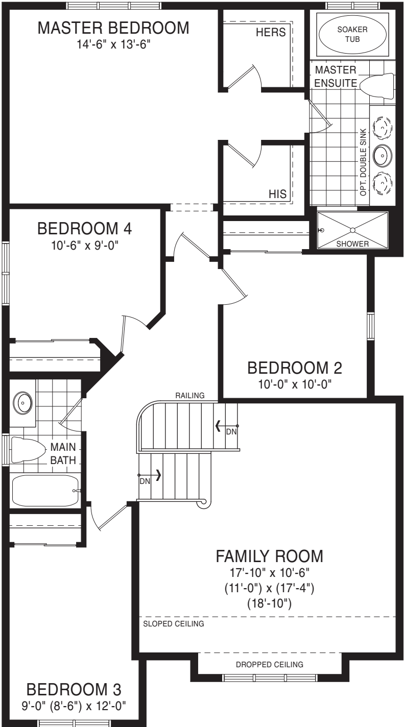
SECOND FLOOR PLAN STYLE A
