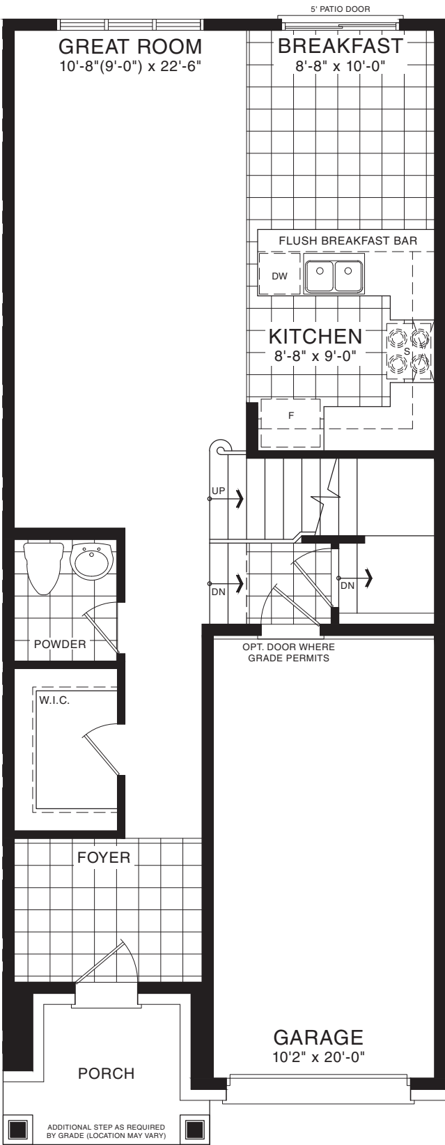
MAIN FLOOR PLAN STYLE A1
