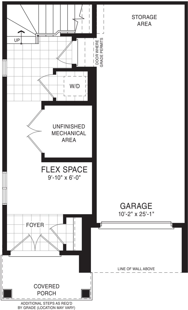
GROUND FLOOR PLAN STYLE A
