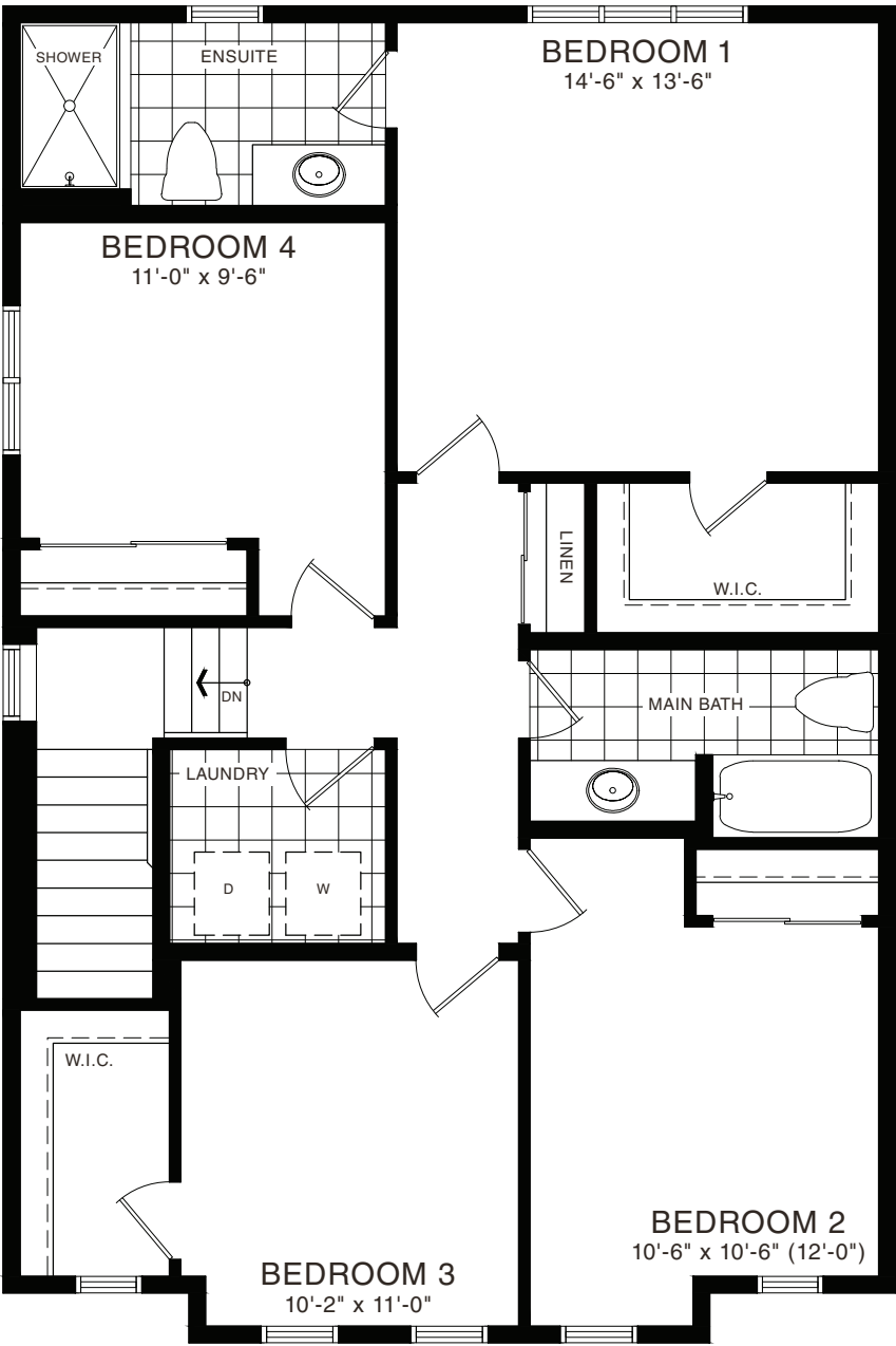
SECOND FLOOR PLAN STYLE A
