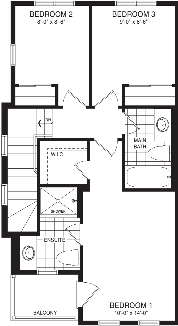
THIRD FLOOR PLAN STYLE A1
