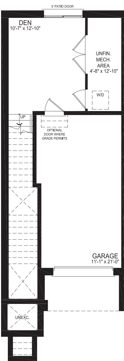
GROUND FLOOR PLAN STYLE A1
