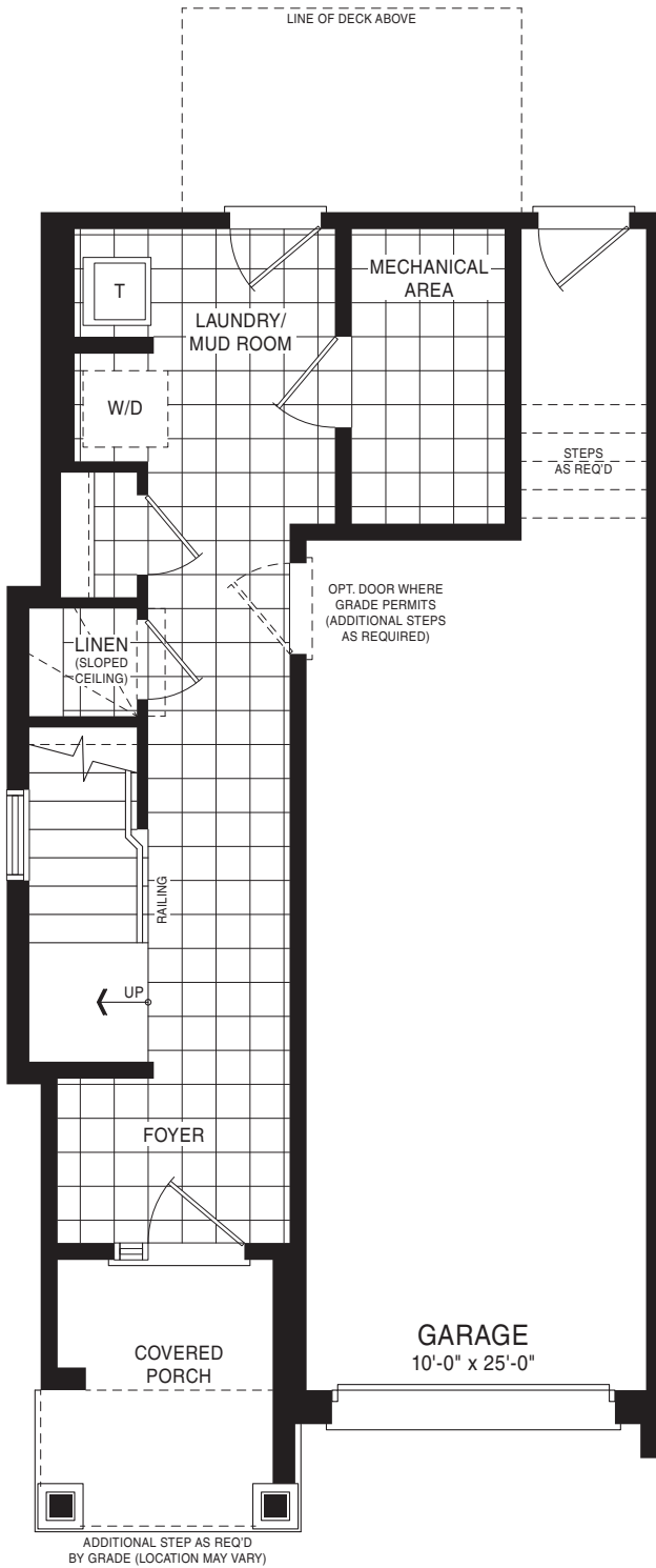
GROUND FLOOR PLAN STYLE A1
