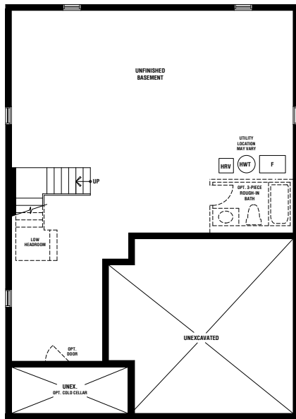
BASMENT PLAN ELEV. 'A'
