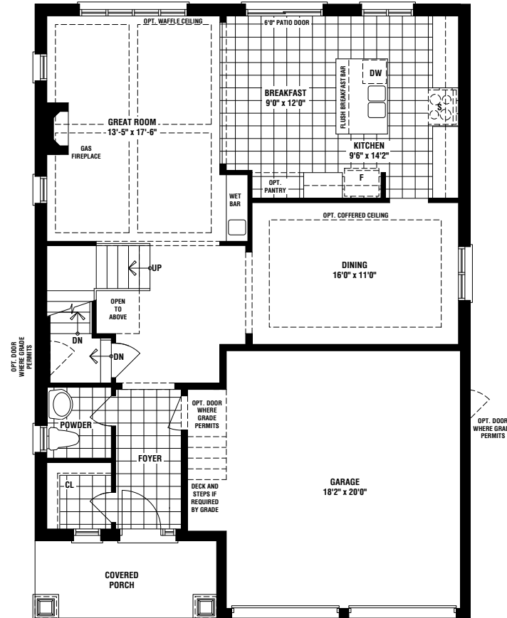
GROUND FLOOR PLAN ELEV. 'A' 9'0" CEILING
