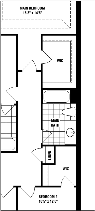
PARTIAL SECOND FLOOR PLAN W/ OPTIONAL GROUND FLOOR LAUNDRY ELEVATION 'A' & 'B'
