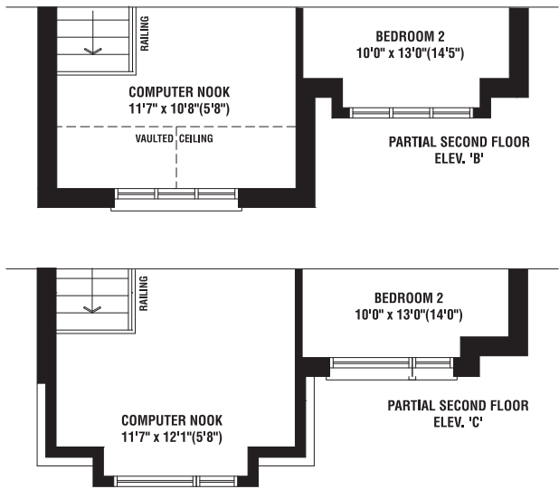
SECOND FLOOR ELEV. 'A'
