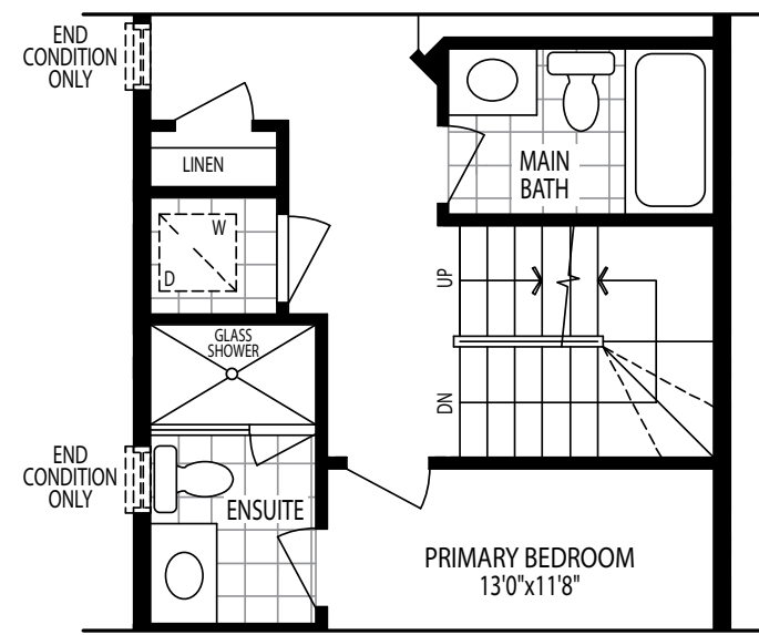
PARTIAL UPPER FLOOR PLAN FOR OPT. ROOF TERRACE ELEV. A1
