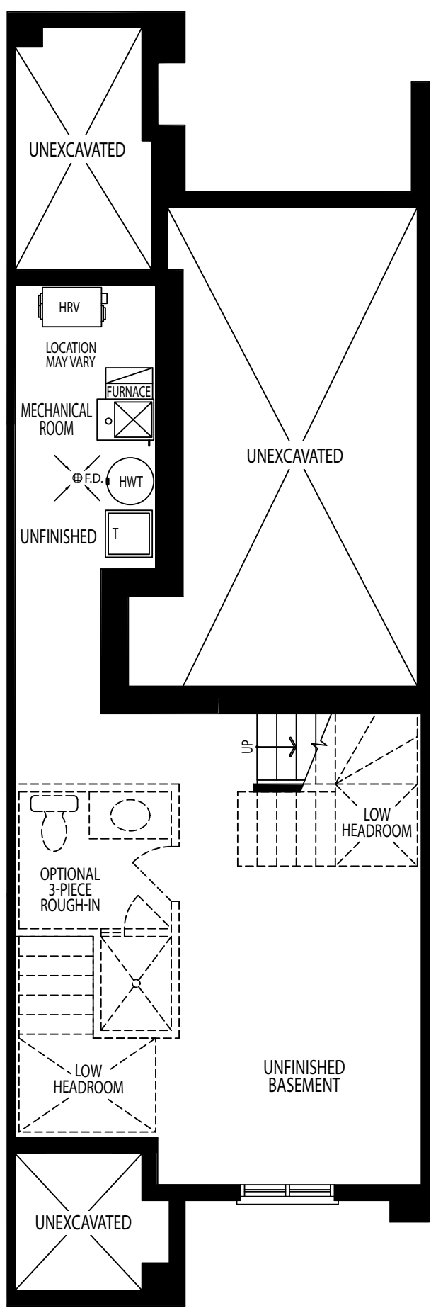
BASEMENT PLAN SUNKEN FRONT FOYER CONDITION ELEV. A1
