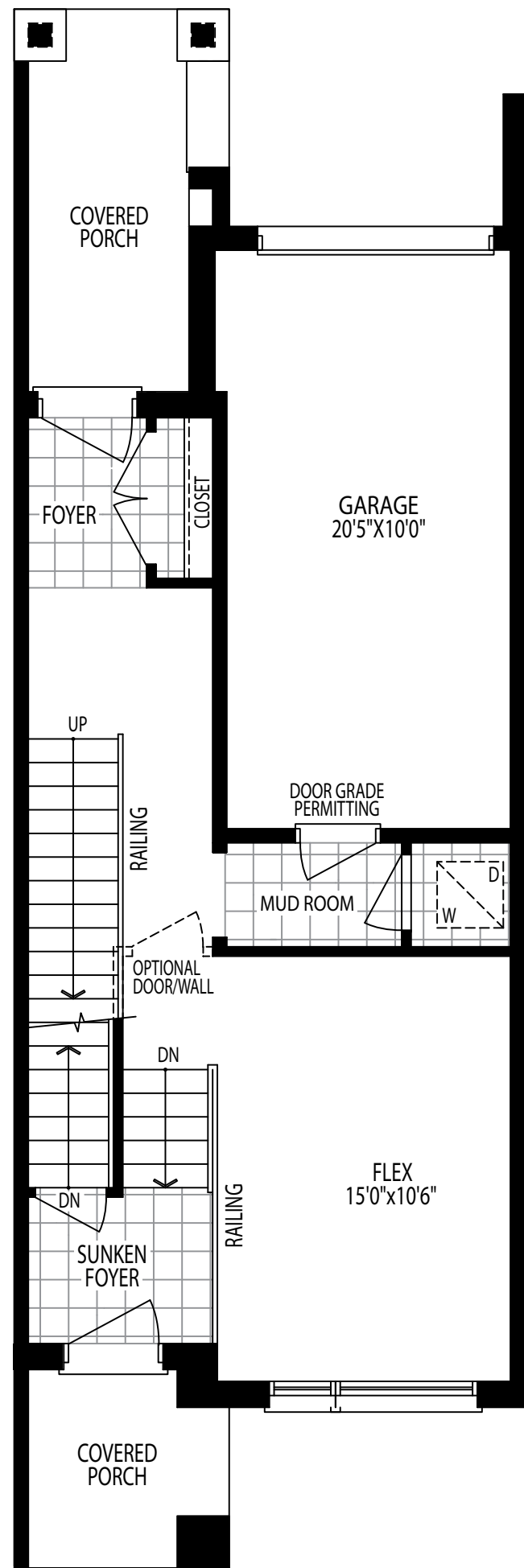
GROUND FLOOR PLAN ELEV. A1
