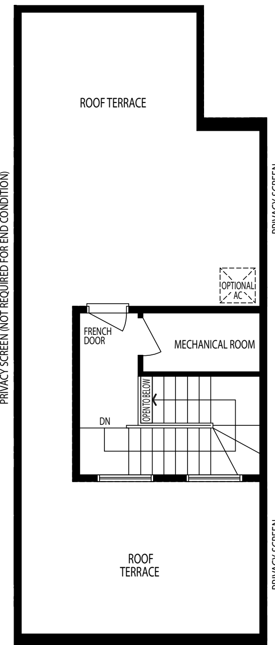
OPT. ROOF TERRACE ELEV. A1
