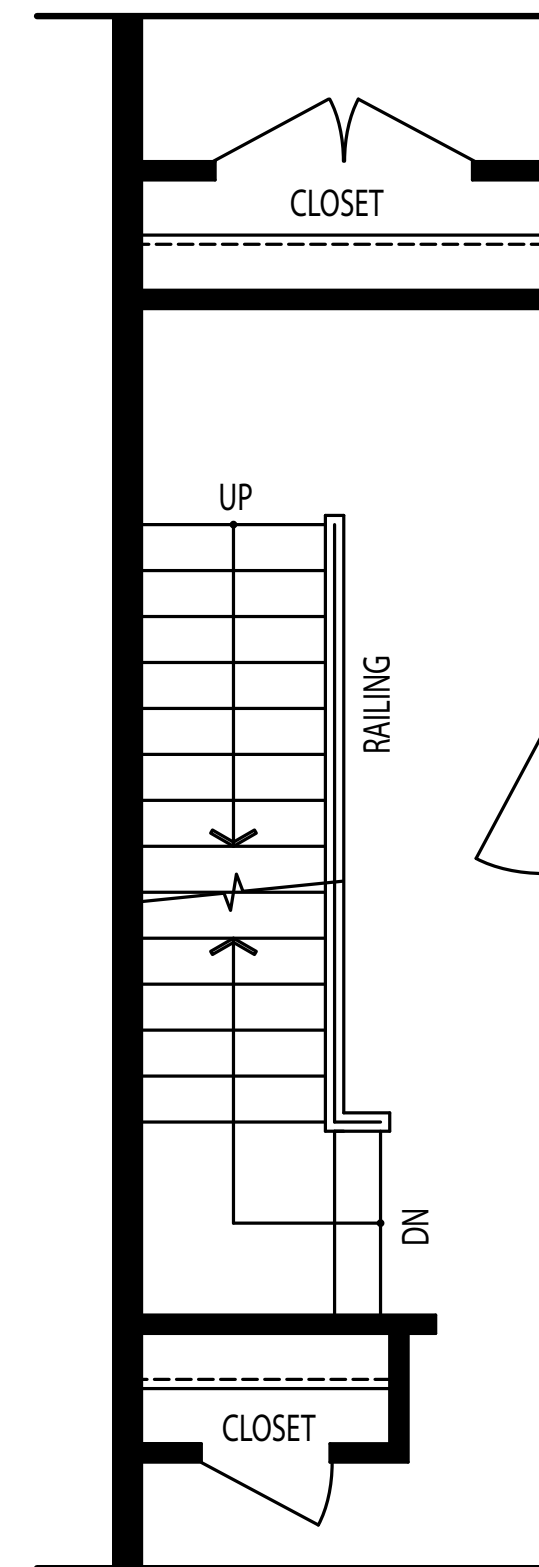
PARTIAL UPPER FLOOR PLAN FOR OPT. ROOF TERRACE ELEV. A
