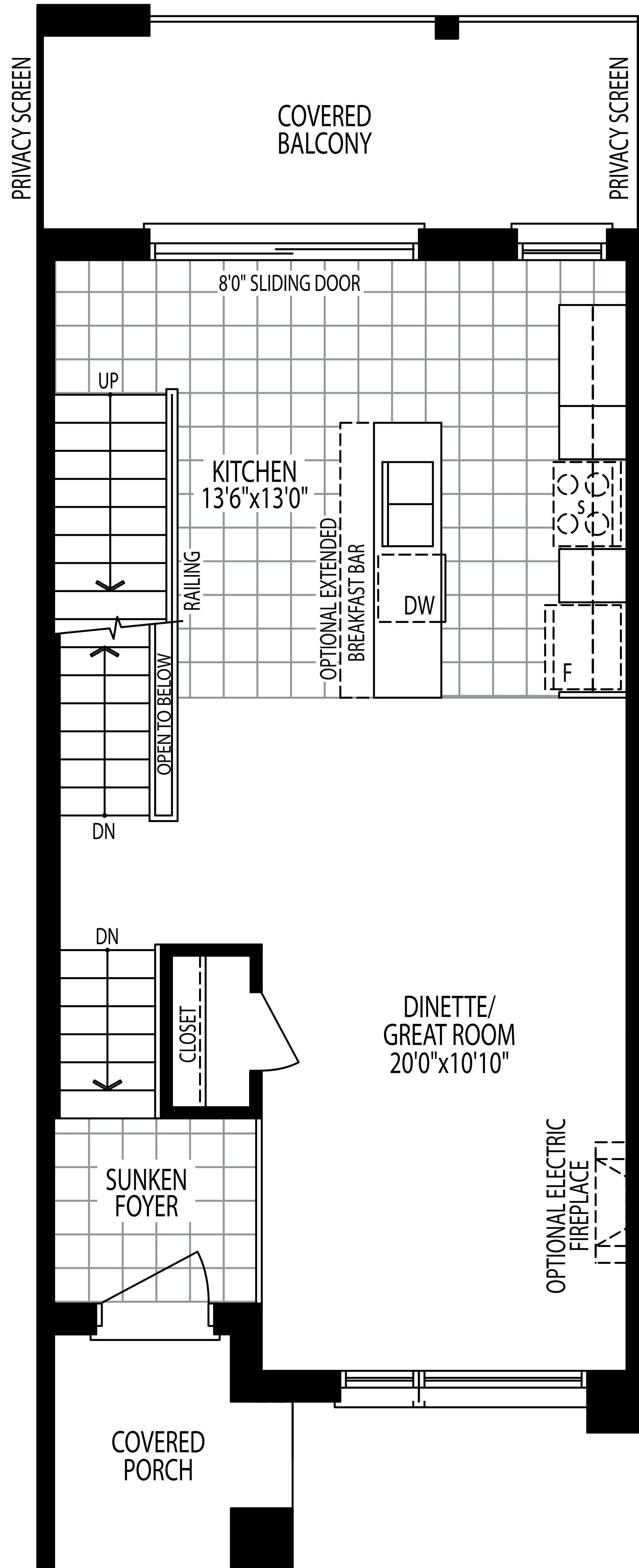
MAIN FLOOR PLAN ELEV. A1
