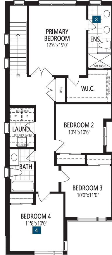
Second Floor
