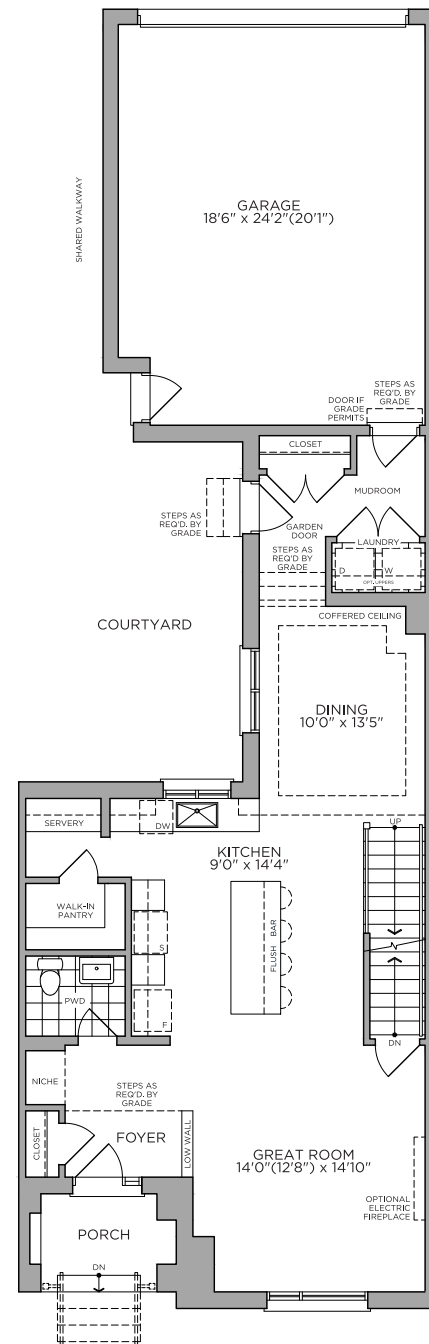
First Floor ELEVATION B
