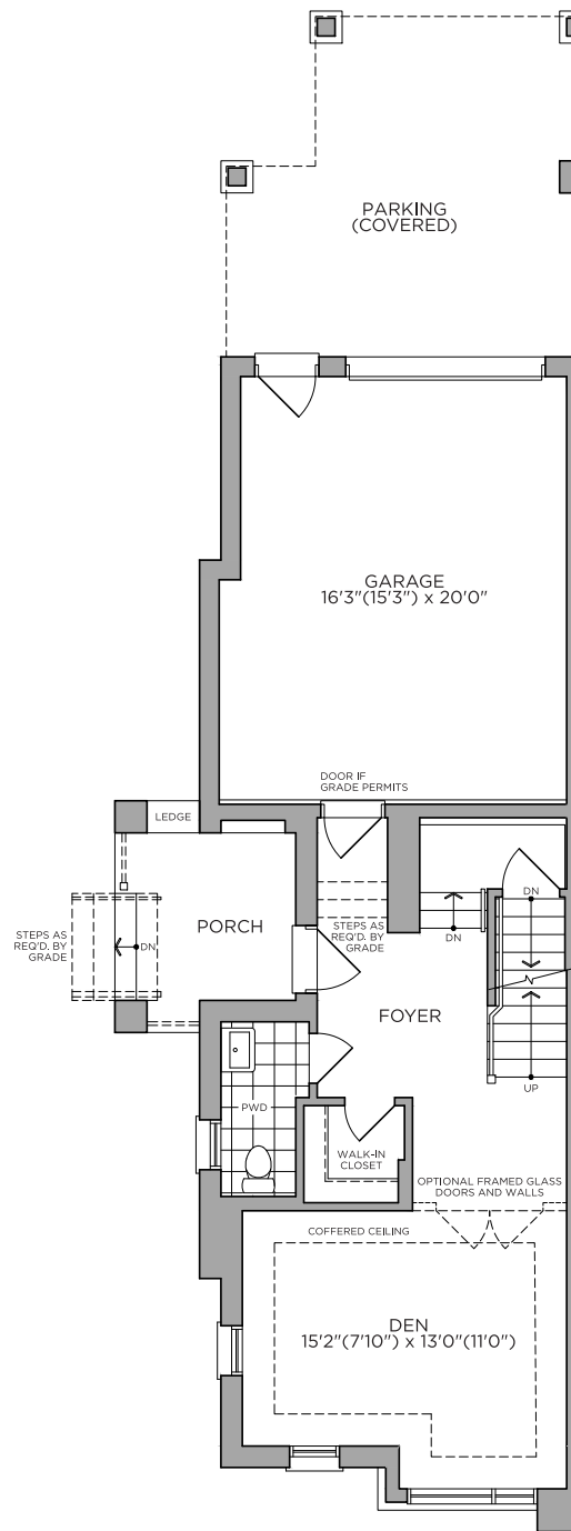
First Floor ELEVATION A, B
