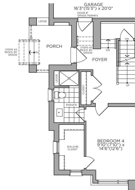
Optional First Floor BEDROOM 4 - ELEVATION A, B
