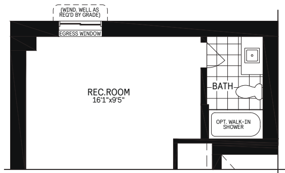
5 Finished Basement Bathroom
