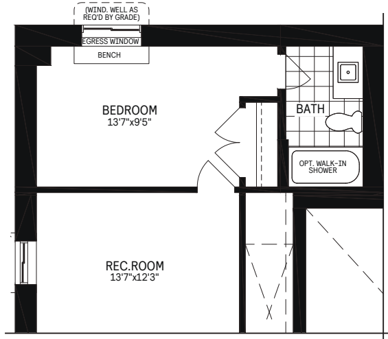
5 Finished Basement Package
