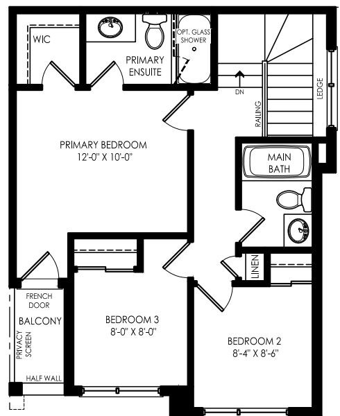
THIRD FLOOR ELEV. B (OPTIONAL 2 ND BATHROOM)
